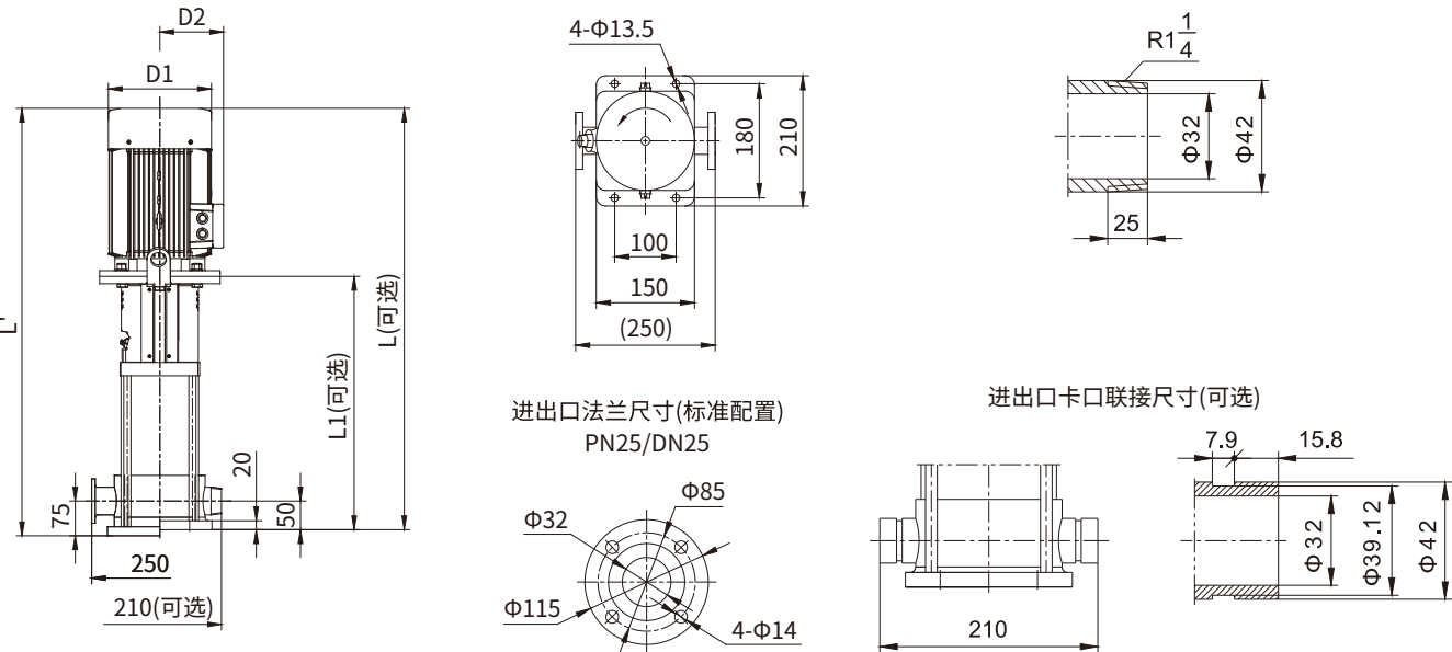
KQDQ25-2安装图
