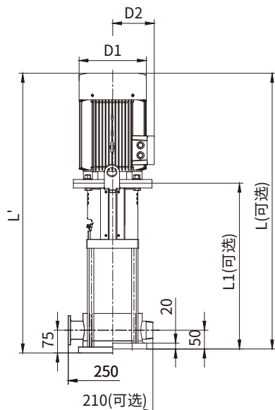
KQDQ32-5安装图
