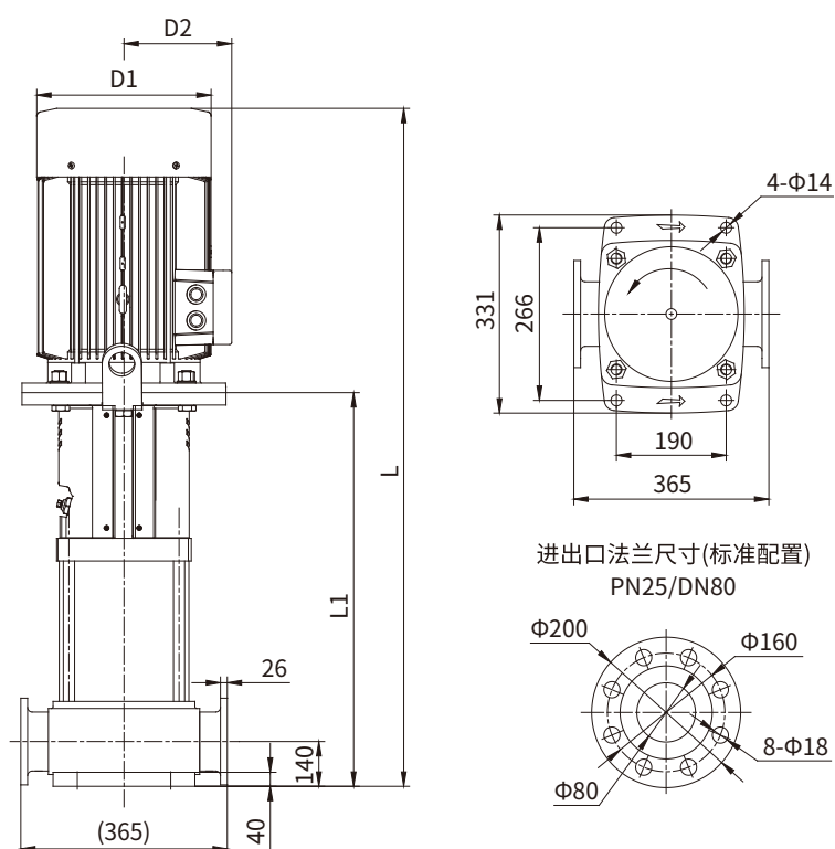
KQDQ80-45尺寸表
