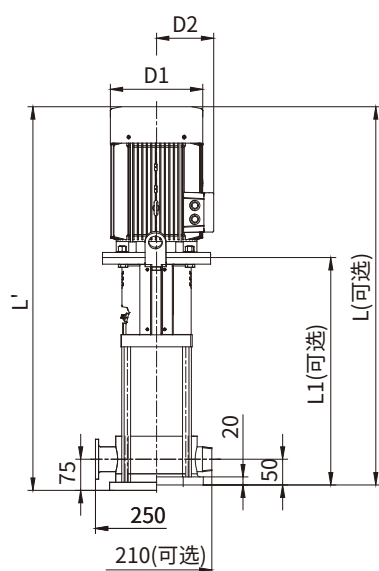
KQDQ25-3安装图
