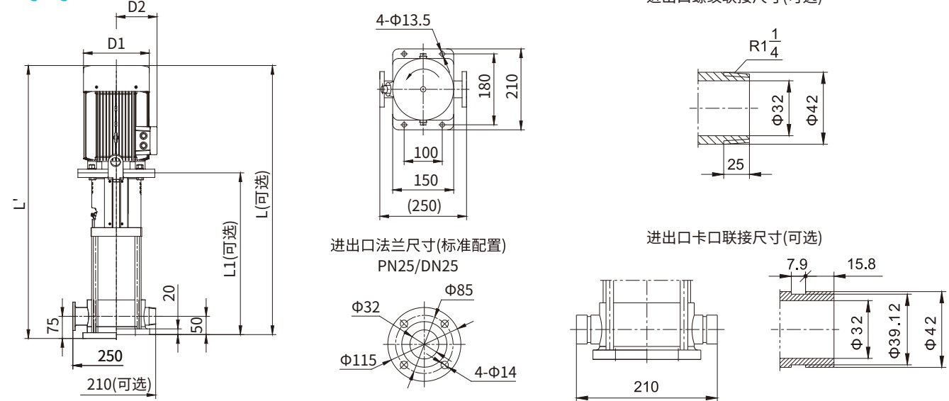
KQDQ25-3G安装图
